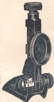
B.S.A. No. 8 Rear Sight. Price 21/6
